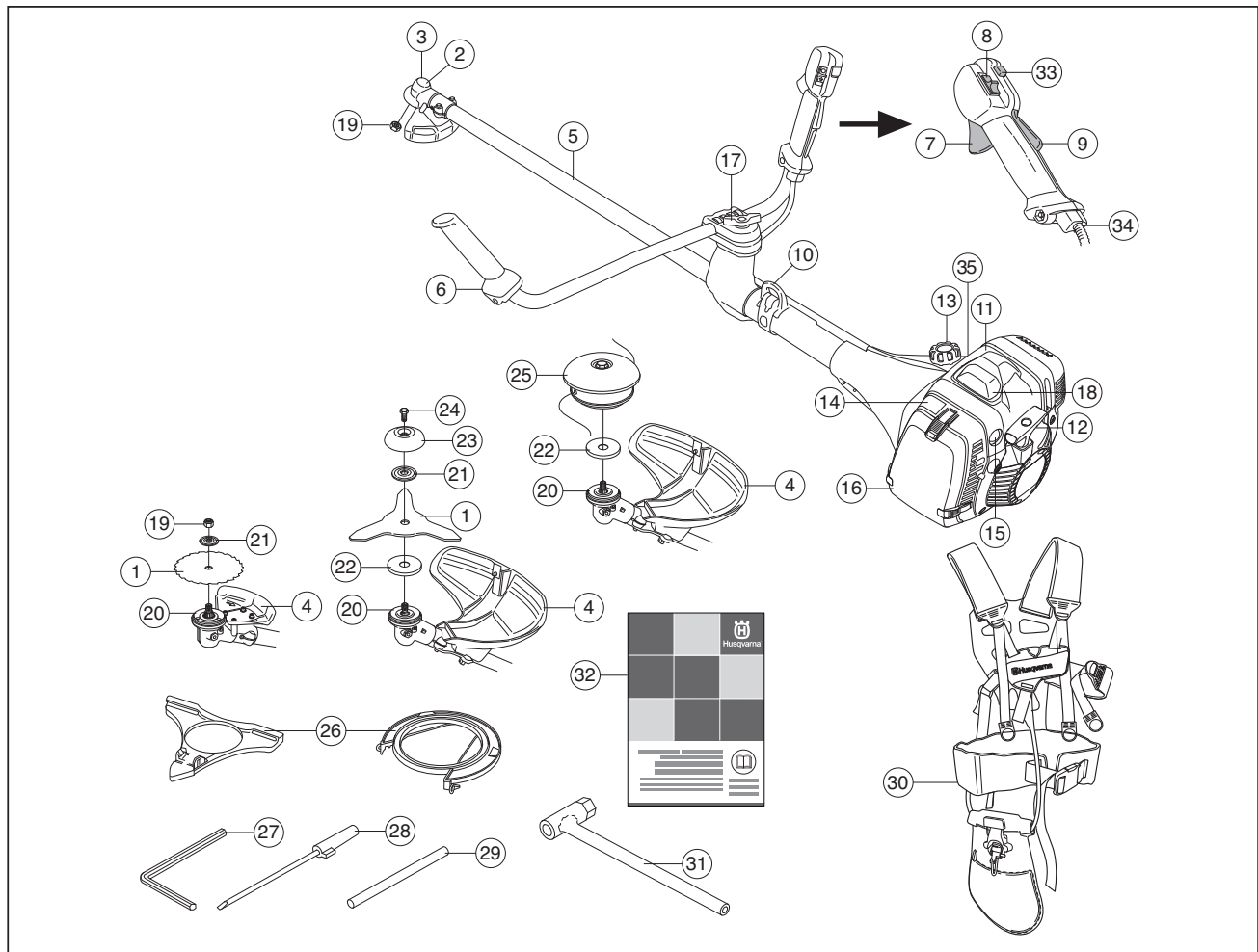
What is what on the brush cutter? (345 FR)
